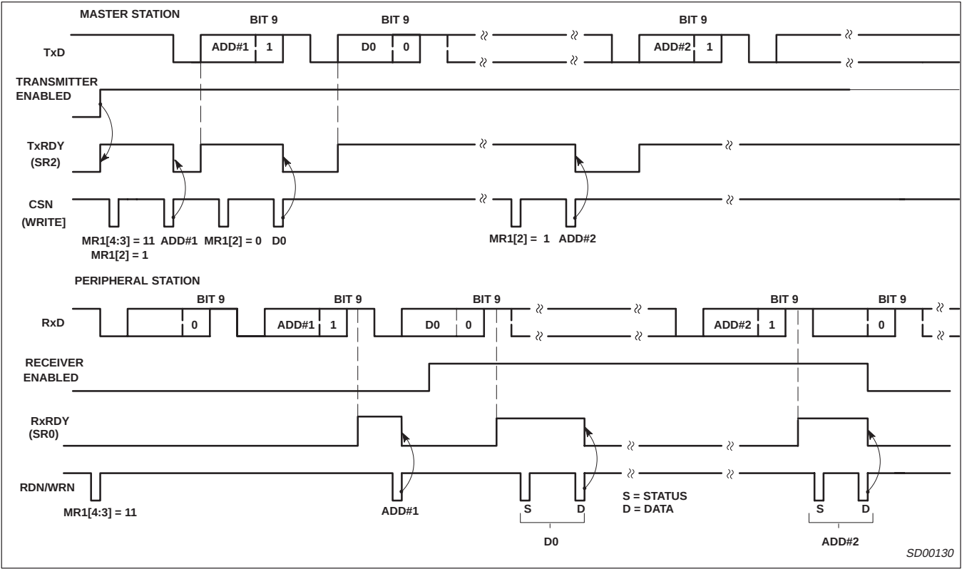
Figure 14. Wake-Up Mode
